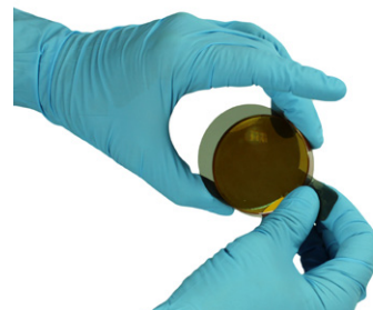
Figure 3b. Uneven coloration indicates mechanical or thermal stress and potential failure. Lens replacement is recommended.
